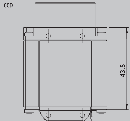
Scale 1:1 (GigE uEye SE) – 3D CAD data on request
